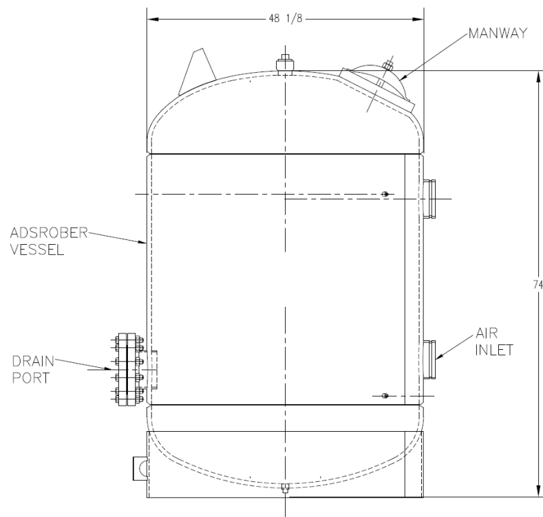
FIG 1: ADSORBER VESSEL GENERAL LAYOUT
