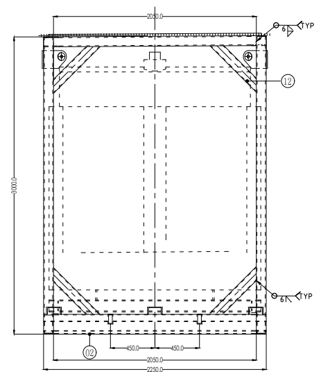
VIEW B-B
