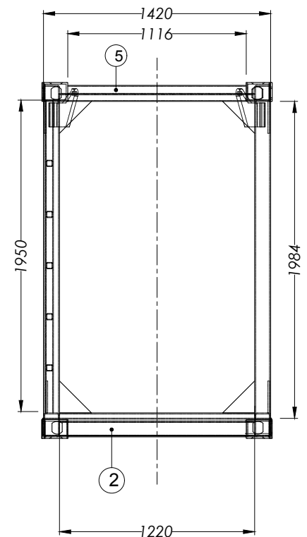
VIEW B-B
